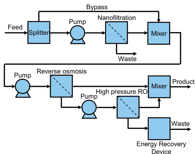
Figure 1. Example ProteusLib flowsheet of a water treatment train including nanofiltration pretreatment and conventional and high pressure reverse osmosis desalination that can be cost optimized subject to constraints on gypsum scaling.
