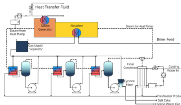
Figure 1. Architecture of a heat integrated multi-effect brine concentrator to be designed and optimized.
