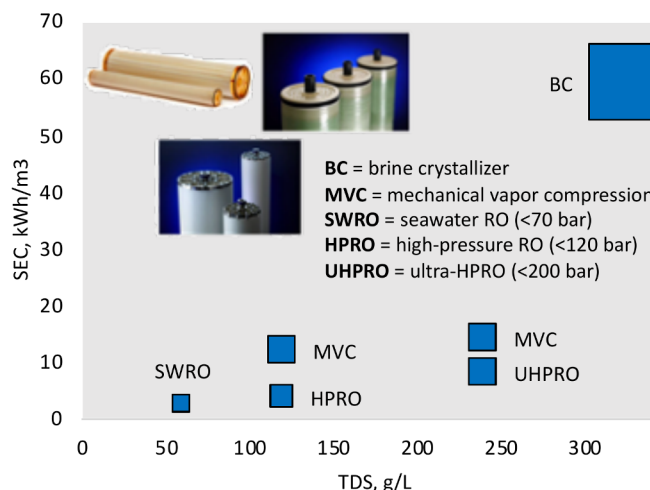
Figure 1. Specific energy consumption by conventional RO, HPRO, UHPRO, brine concentrator, and brine crystallizer. The specific energies shown in the figure are in kWh per cubic meter of feedwater.
