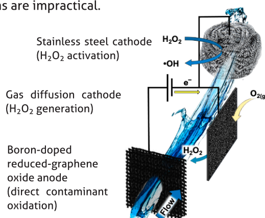
Figure 1. Schematic of the envisioned 3-electrode system for simultaneous contaminant oxidation and in-situ hydrogen peroxide generation.
