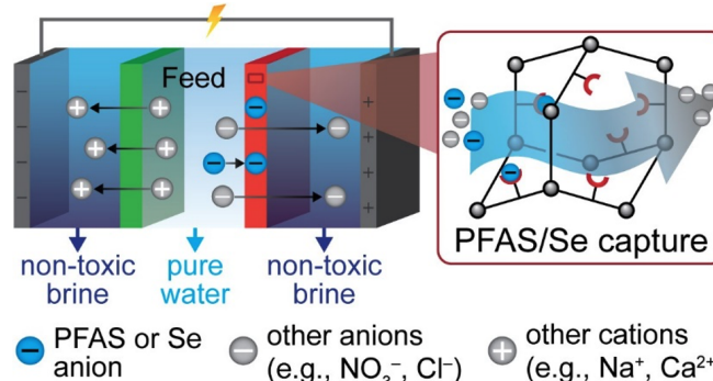
Figure 1. Simultaneous water desalination and selective PFAS or selenium capture by ion-capture electro dialysis, using anion-conductive membranes embedded with selective PPN adsorbents.
